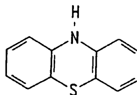
Phenothiazine
